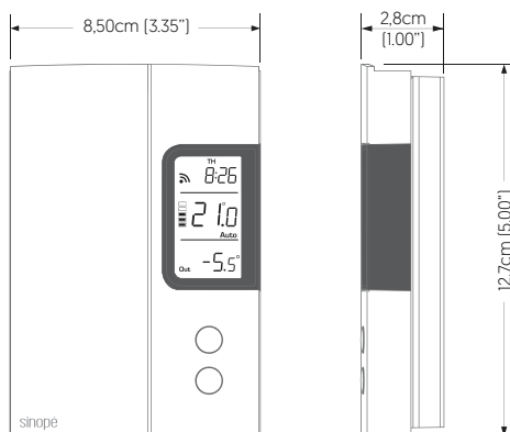
TH1120RF-3000
