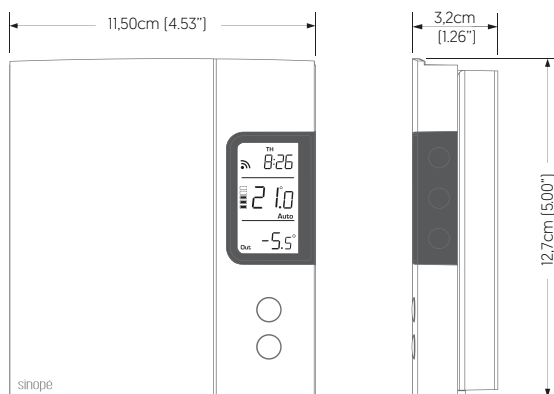
TH1120RF-4000
