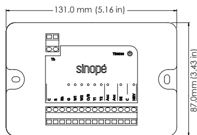
Connection module [TB6500]
