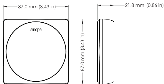
Thermostat
